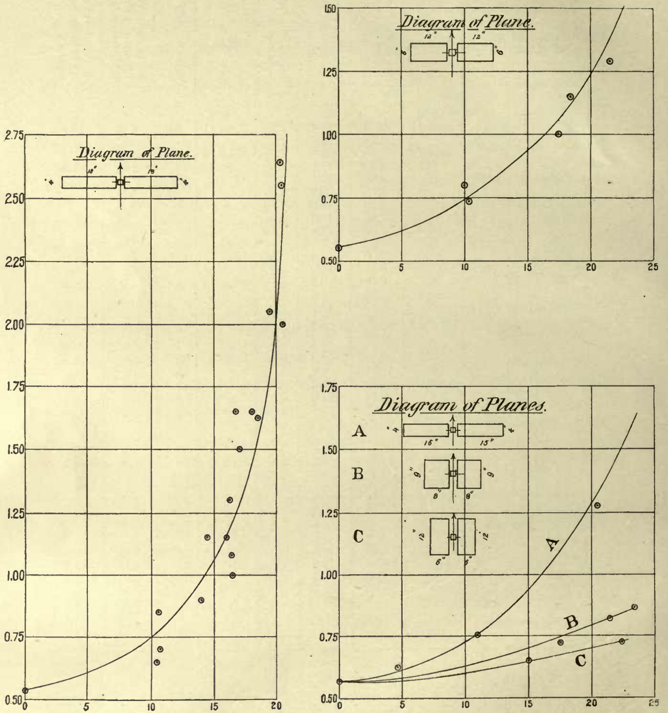
Times of falling 4 feet of horizontal planes on the Plane-Dropper . Average weight of planes = 465 grammes. Abscissæ : = Horizontal velocities of translation in meters per second. Ordinates : = Times of fall in seconds.
